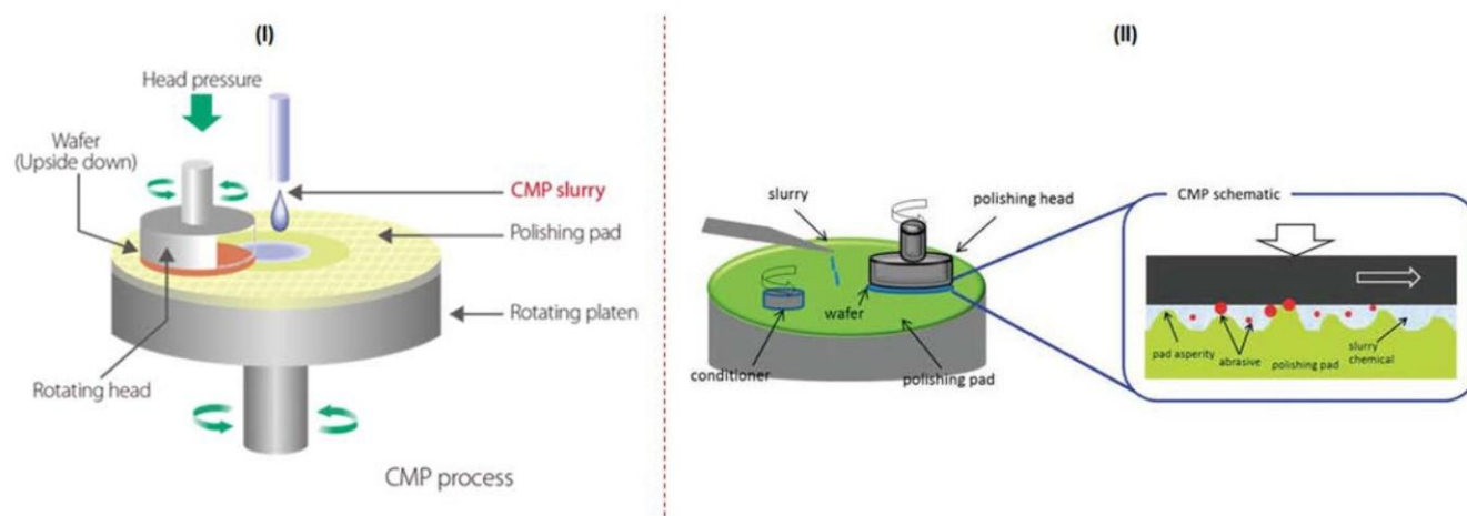
Fig. 135: CMP process
