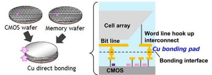
Fig. 94: The wafer-to-wafer bonding structure
