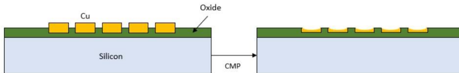
Fig. 84: CMP process of SoIC
