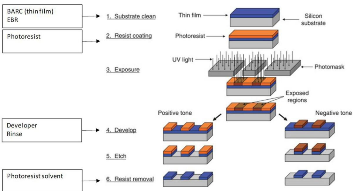
Fig. 126: Photoresisting processes
