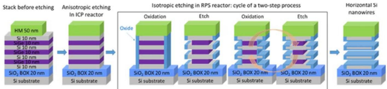
Fig. 74: Process of forming the GAA transistor
