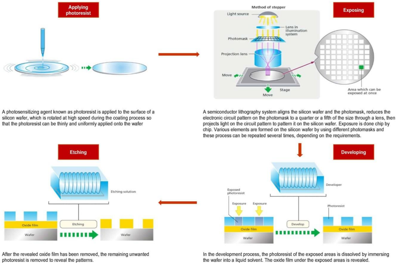
Fig. 125: Photoresist and lithography process
