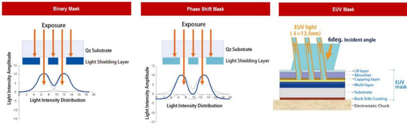
Fig. 129: Photomask classification
