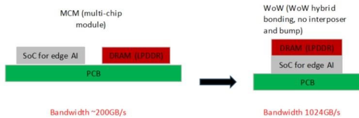
Fig. 13: Difference between MCM vs WoW for edge AI chips
