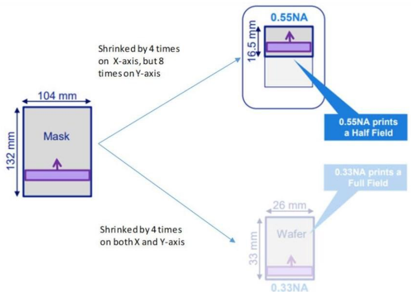
Fig. 59: Half-field printed chips vs full-field printed chips – 2
