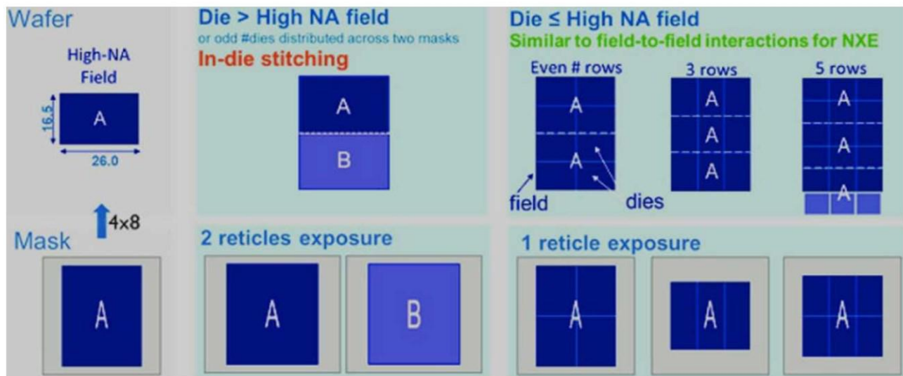
Fig. 65: High-NA EUV process for large and small die size ICs
