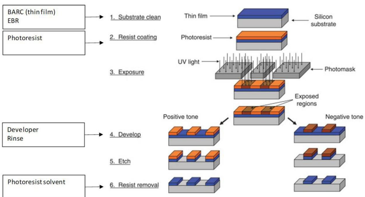
Fig. 156: PR processes and the materials required
