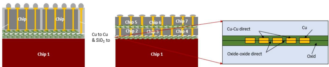
Fig. 83: Chip to chip/wafer hybrid bonding
