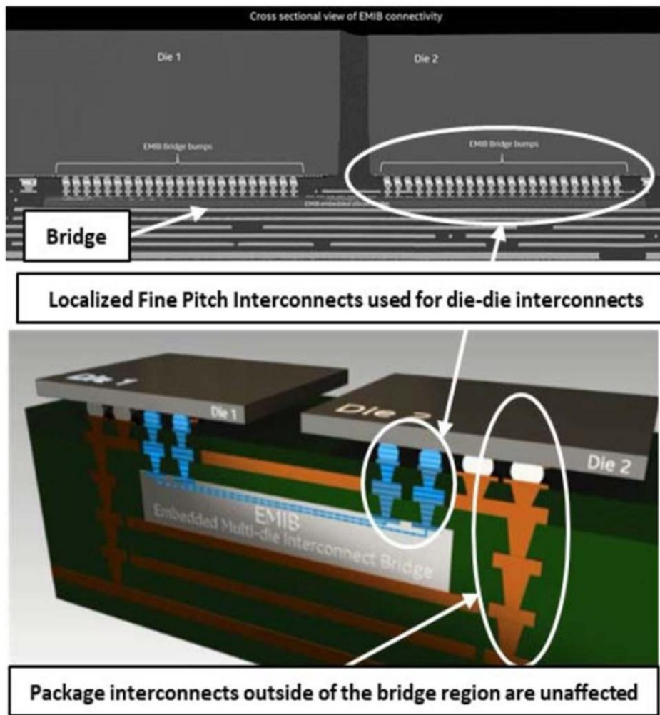
Fig. 104: An illustration of EMIB
