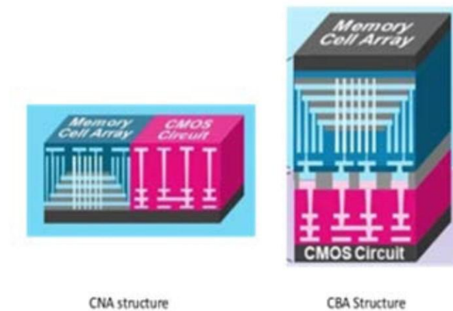
Fig. 180: 3D NAND: CNA vs CBA structure
