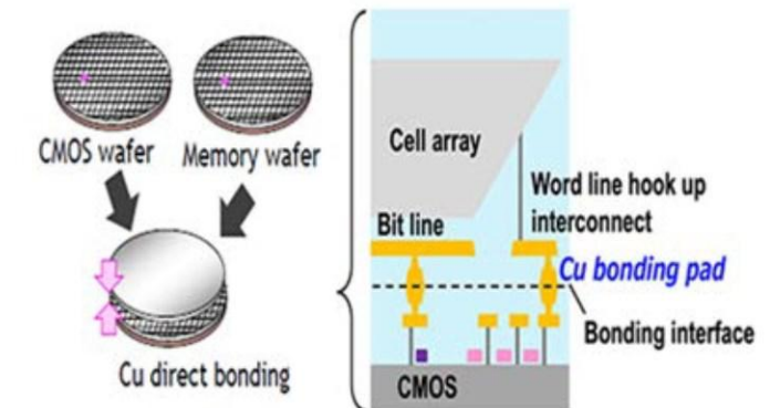
Fig. 181: The wafer-to-wafer bonding structure
