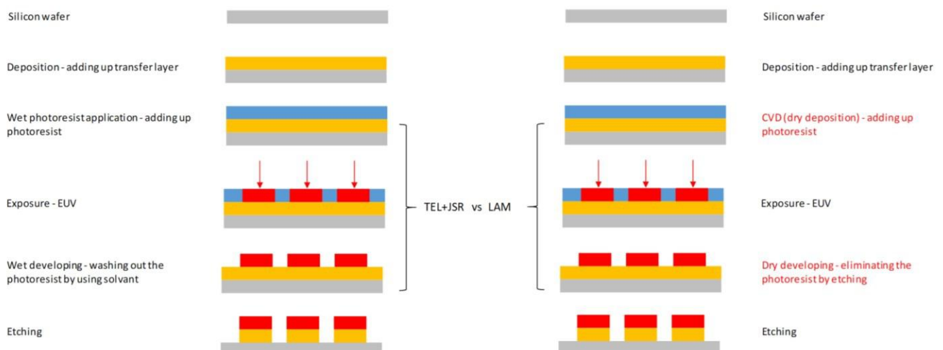
Fig. 63: TEL and JSR vs Lam Research's solution
