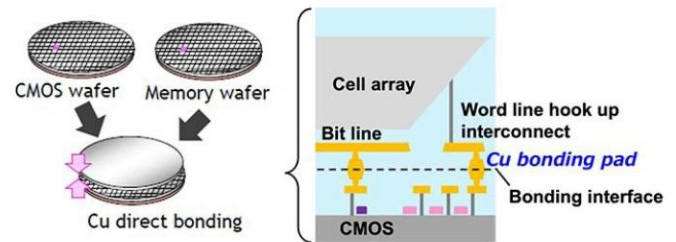
Fig. 11: Wafer-to-wafer bonding structure
