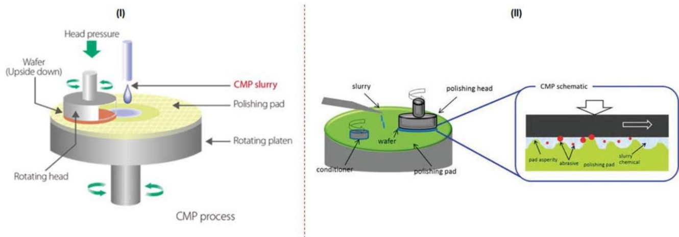
Fig. 135: CMP process
