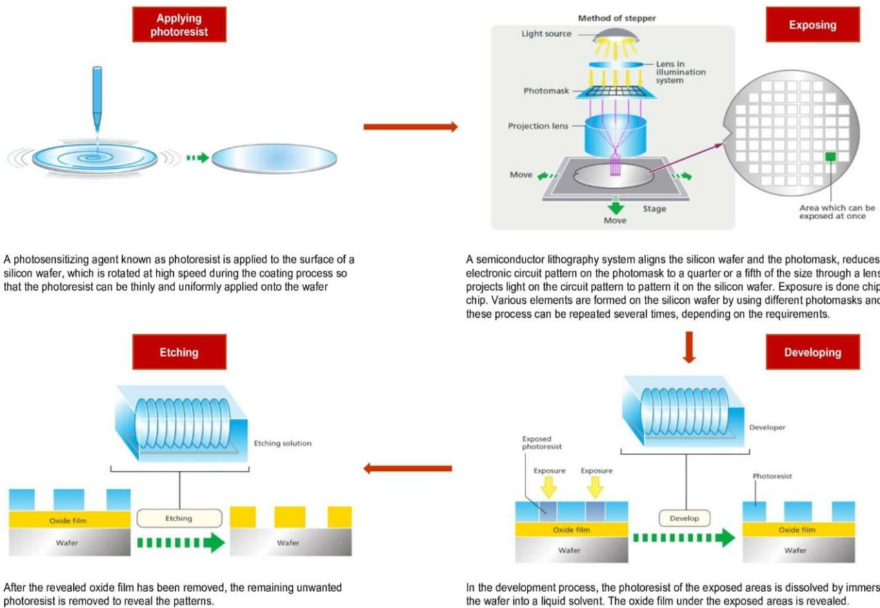
Fig. 155: PR and lithography process
