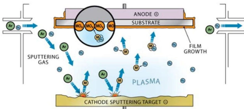
Fig. 139: Sputtering process
