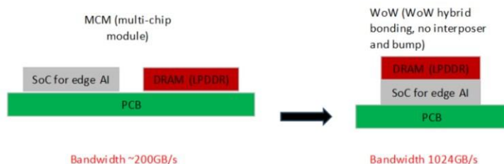
Fig. 100: Difference between MCM vs WoW for edge AI chips
