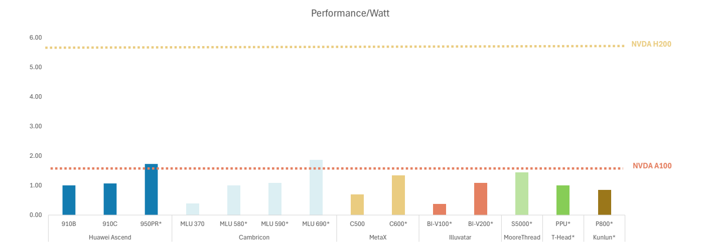
Exhibit 19: Performance/watt comparison
