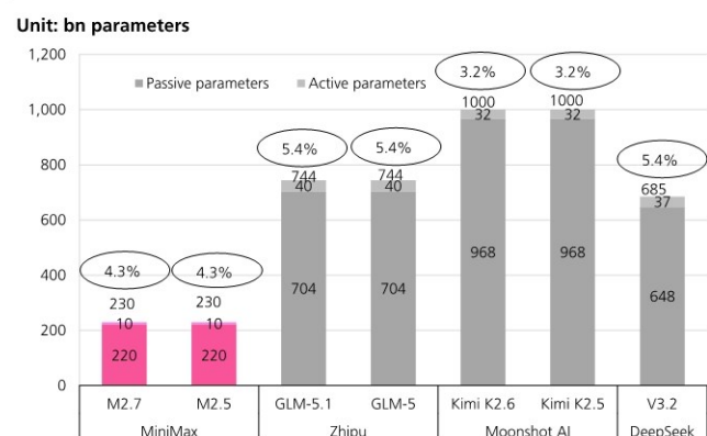
Figure 2: Total parameters and activation rate comparison among models across China's AI labs
