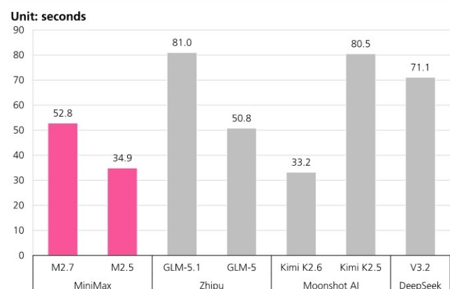
Figure 4: Latency comparison among models across China's AI labs
