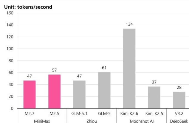
Figure 5: Output speed comparison among models across China's AI labs
